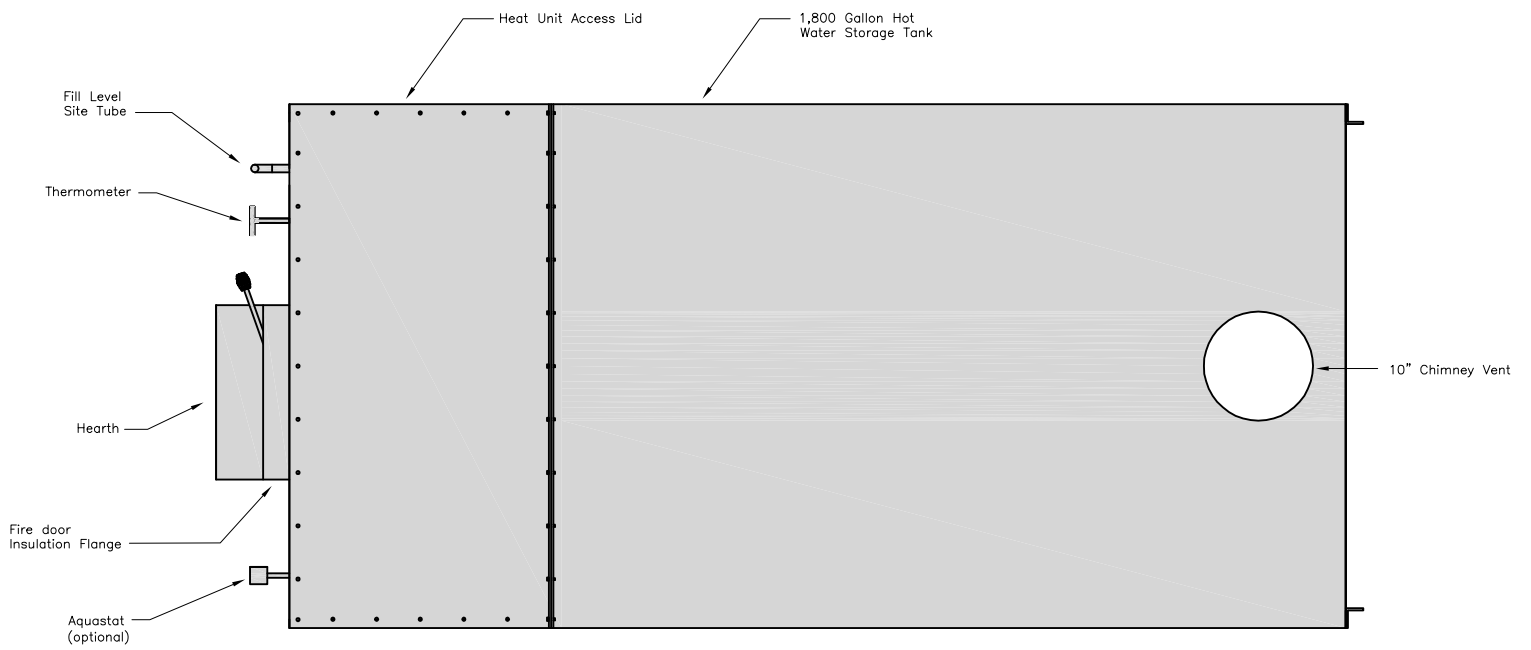
Model TH-4 Top View
