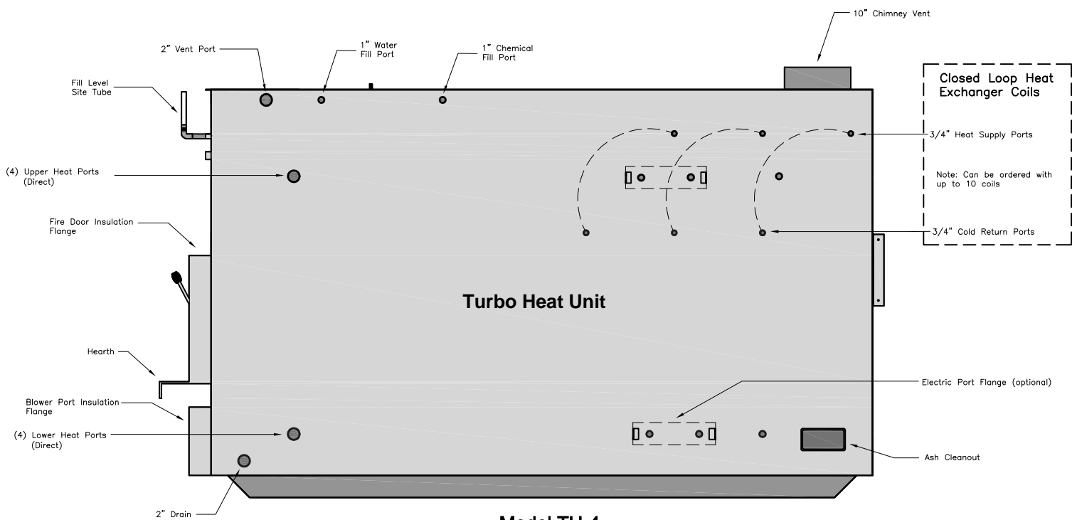
Model TH-4 Right Side View
