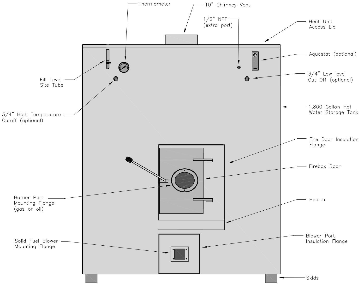
Model TH-4 Front View
