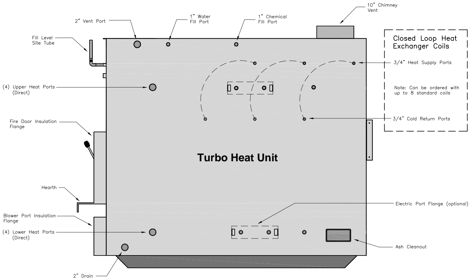
Right Side View Model TH-3
