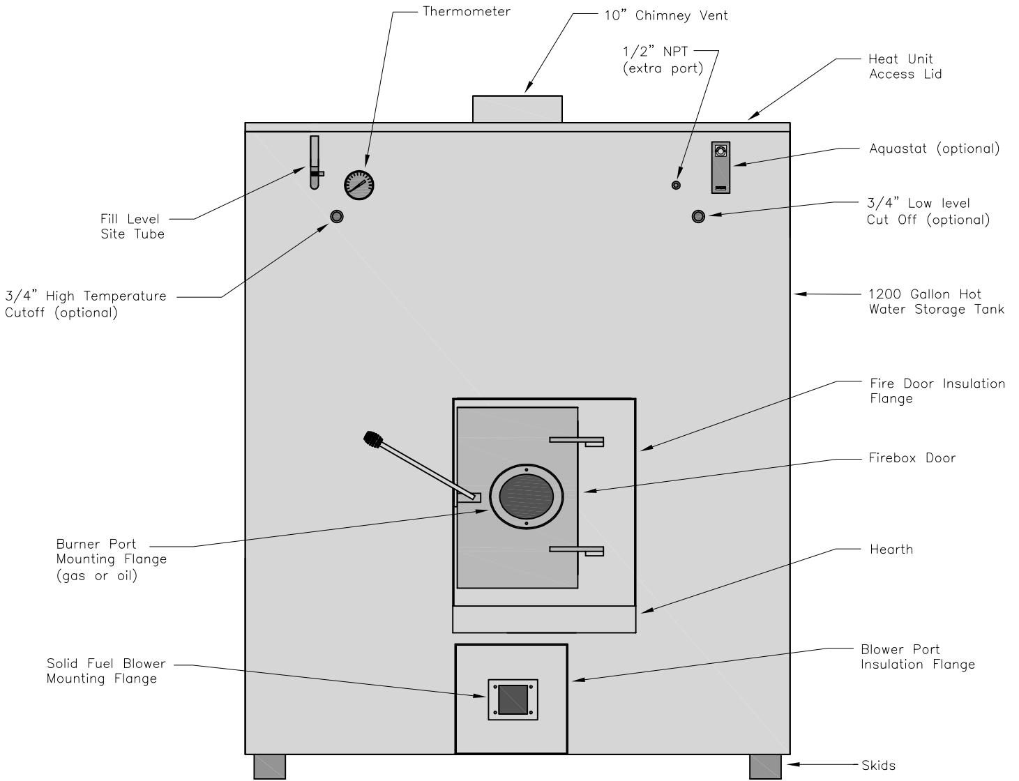
Model TH-3 Front View
